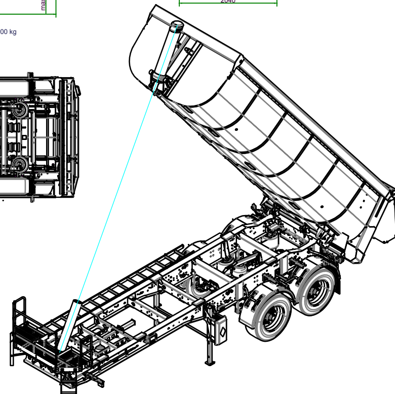
Drawn SH 1200-1250 TRH470 LH1500
